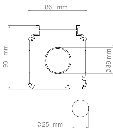
Screen case, side view (ø39 mm bar)
