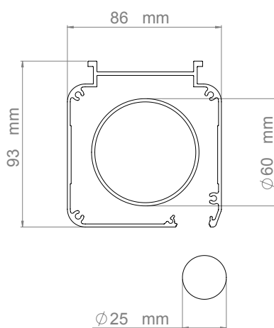
Screen case, side view (ø60 mm bar)
