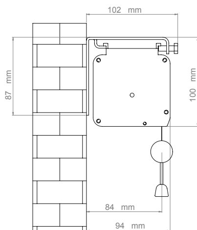
Wall mounting
