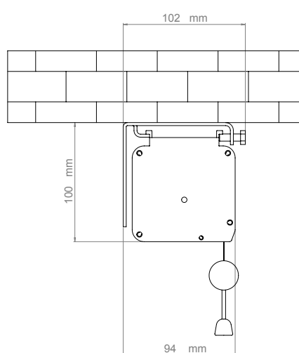
Ceiling mounting
