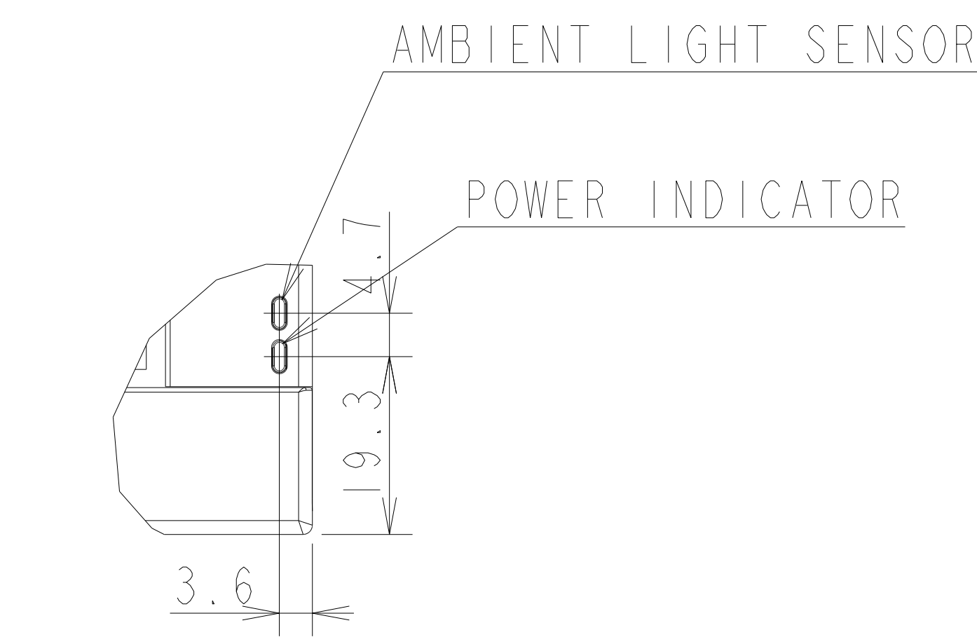
DETAIL A
